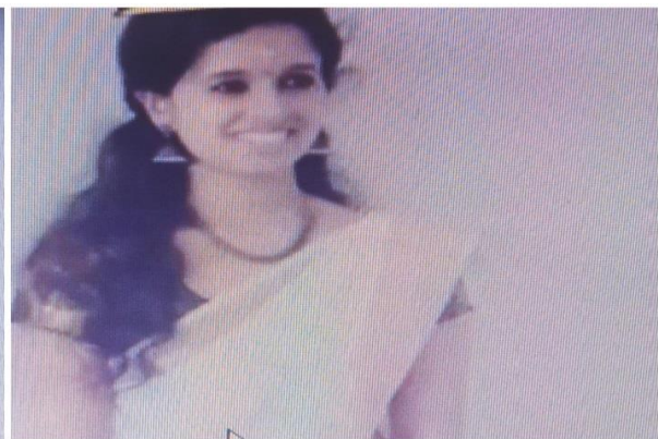
Nutrigirl competition
